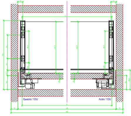
AVT YOU with Aluminum Profile
