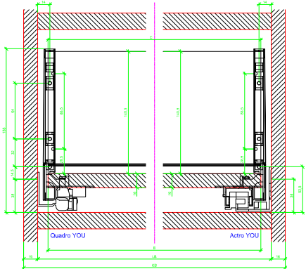
AVT YOU with Aluminium Profile
