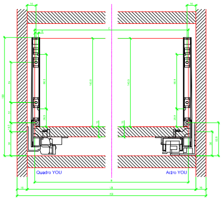
AVT YOU with Wooden Panel
