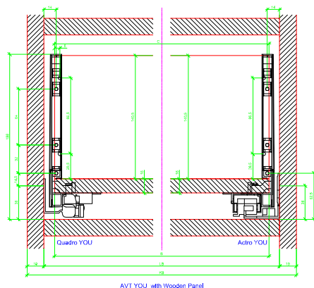
AVT YOU with Wooden Panel
