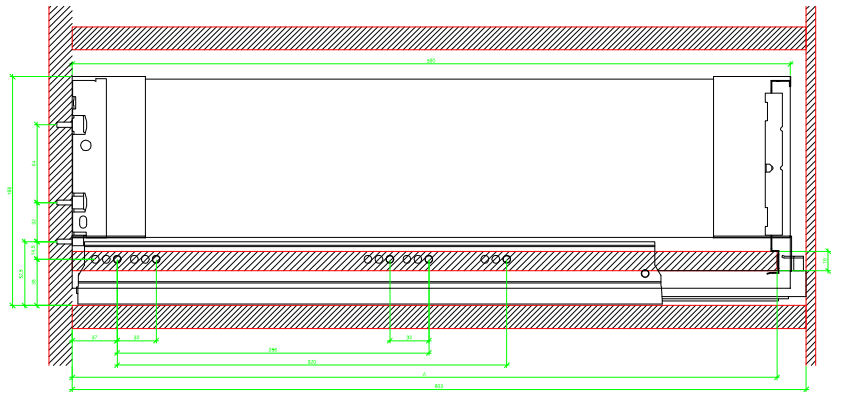
AVT YOU with Steel Rear Panel
