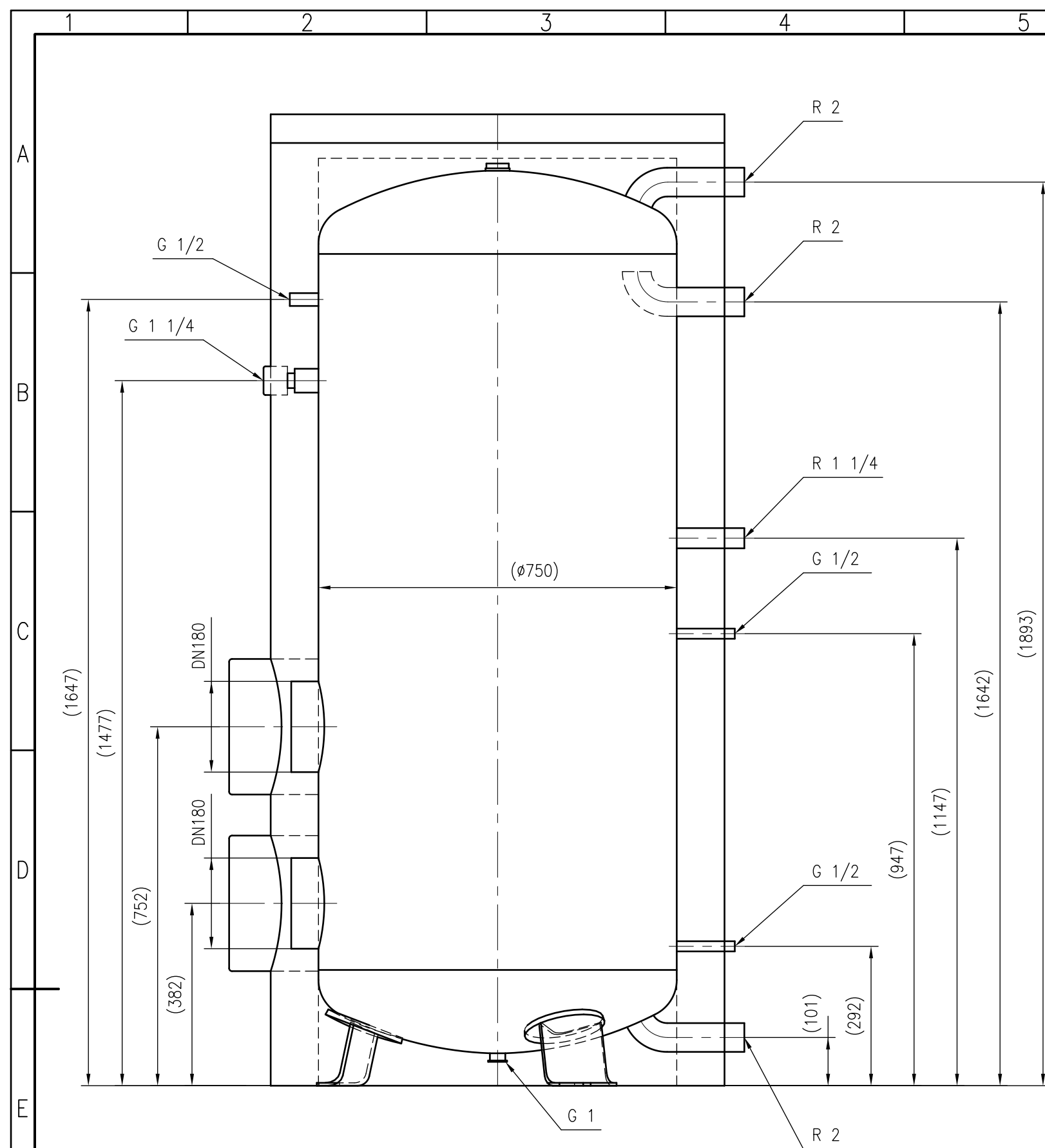
Side view
