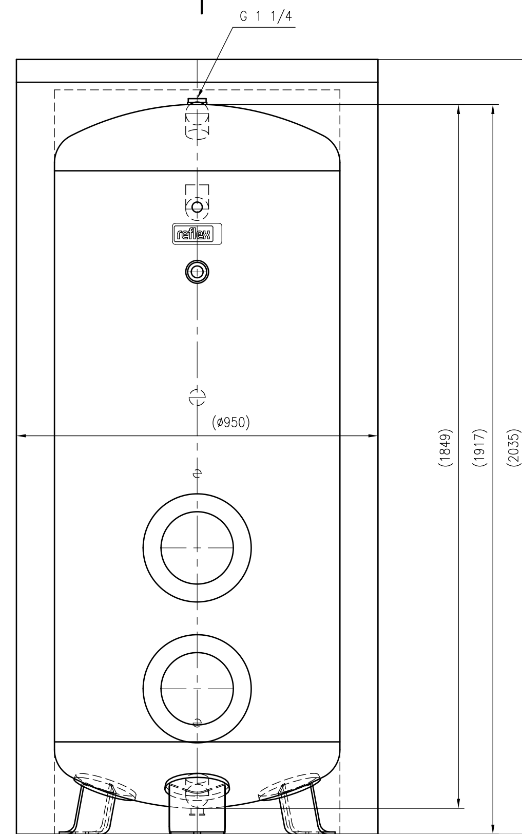
Front view
