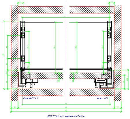
AVT YOU with Aluminum Profile
