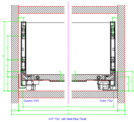
AVT YOU with Steel Rear Panel
