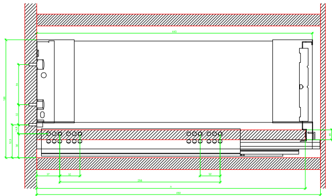
AVT YOU with Steel Rear Panel
