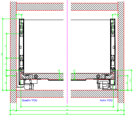
AVT YOU with Steel Rear Panel
