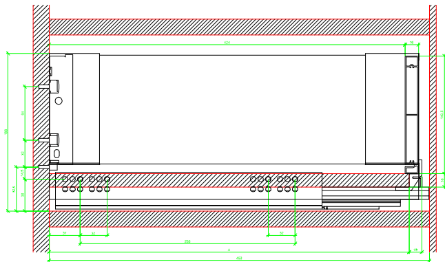
AVT YOU with Aluminum Profile
