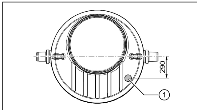
(1) Cable penetration sleeve in EasyClean ground NS 1-4
