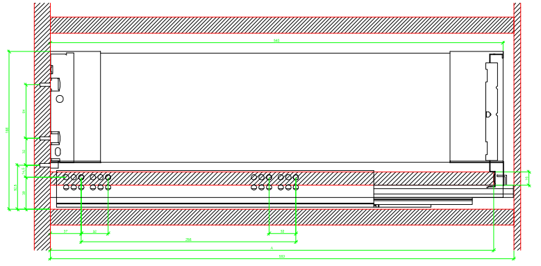
AVT YOU with Steel Rear Panel
