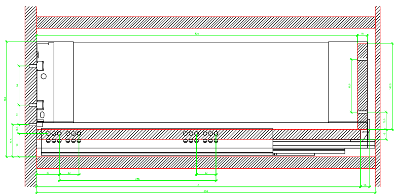
AVT YOU with Wooden Panel
