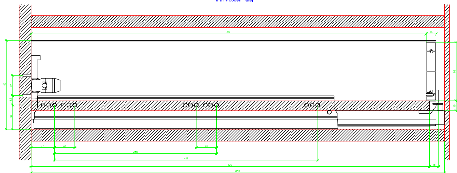
AVT YOU with Aluminium Profile
